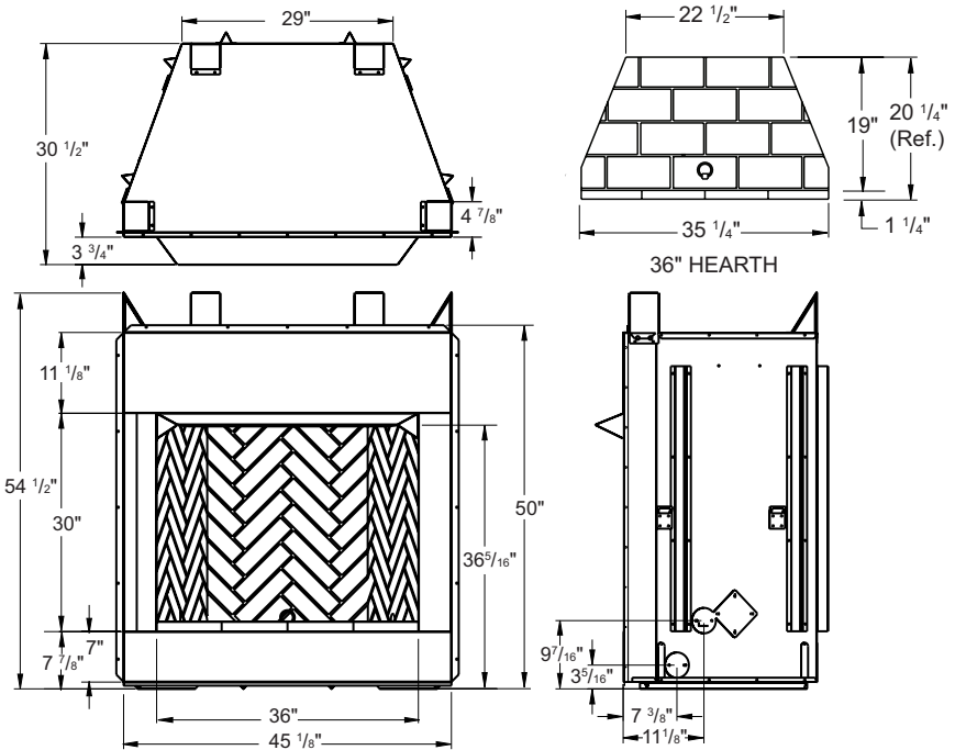
Figure 1 - 36" Models (V)U36(H,S) and (V)Q36(H,S)(R) Series (Picture may vary from actual fireplace)
