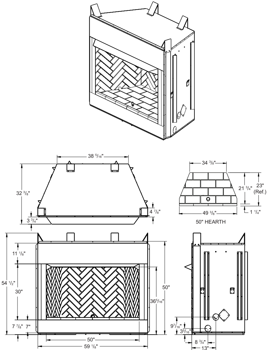
Figure 3 - 50" Models (V)U50(H,S) AND (V)Q50(H,S)(R) Series (Picture may vary from actual fireplace)
