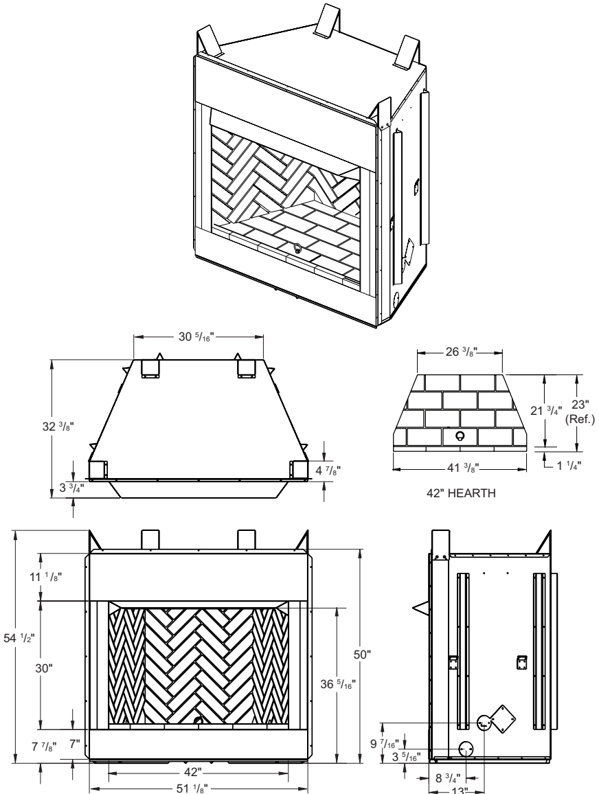
Figure 2 - 42" Models (V)U42(H,S) and (V)Q42(H,S)(R) Series (Picture may vary from actual fireplace)
