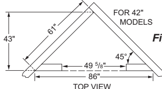
Figure 7 - Rough Opening for Installing in Wall
