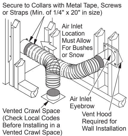
Figure 11 - Outside Air Kit
