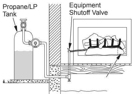
Figure 9 - Checking Gas Joints (Propane/LP Gas Only)
