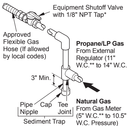
Figure 7 - Gas Connection
