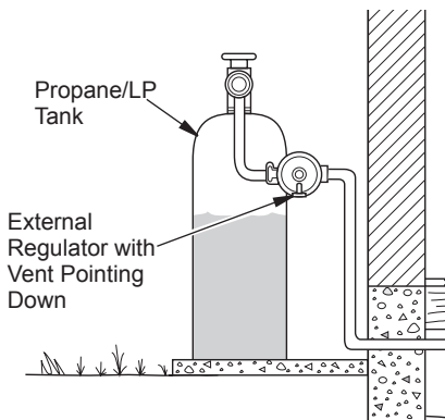
Figure 6 - External Regulator with Vent Pointing Down
