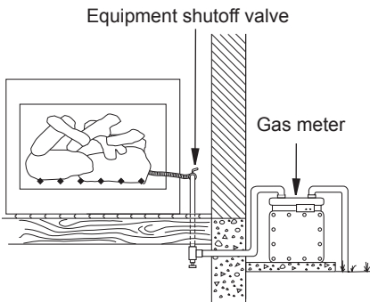
Figure 6 - Checking Gas Joints
