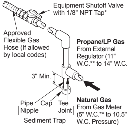
Figure 4 - Gas Connection
