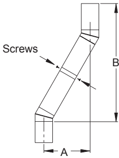
Figure 9 - Elbow Offset
