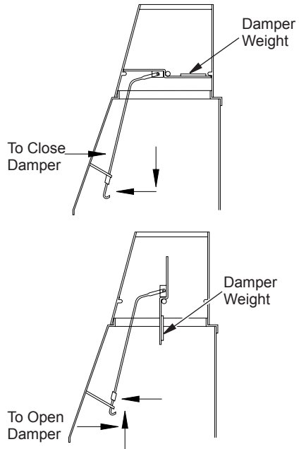
Figure 25 - Operating Damper Handle
