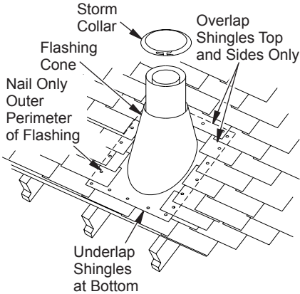
Figure 13 - Flashing Installation
