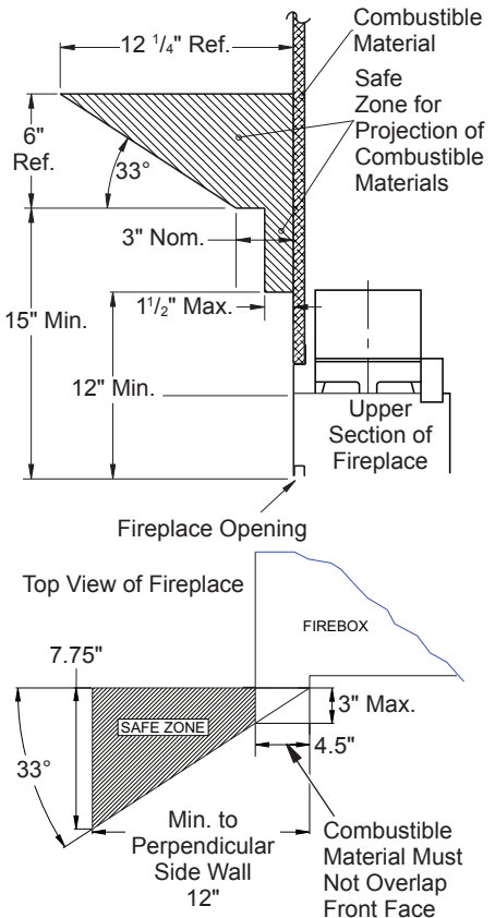
Figure 4 - Mantel Clearances to Combustible Material
