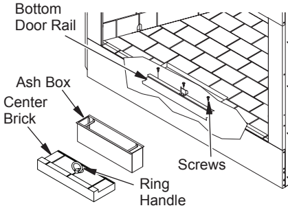
Figure 27 - Installing Bottom Door Frame
