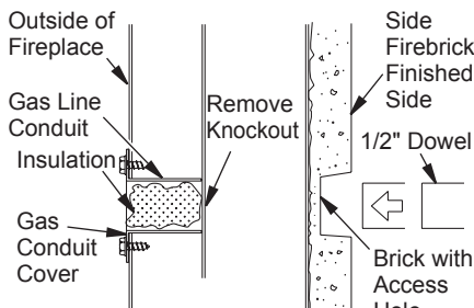
Figure 24 - Gas Line Access
