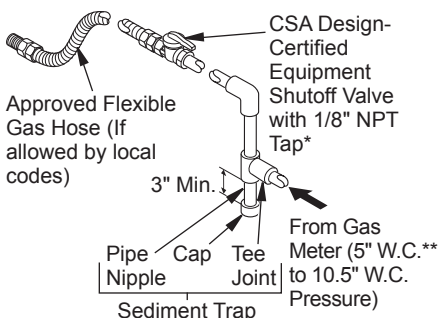
Figure 8 - Gas Connection
