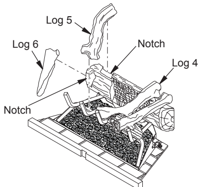
Figure 24 - Installing Logs 5 and 6
