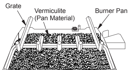
Figure 19 - Fill Entire Burner Pan with Vermiculite
