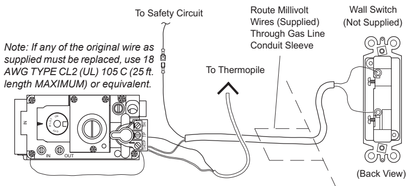
Figure 14 - Wall Switch Wiring Diagram
