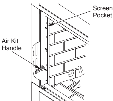
Figure 30 - Air Kit Handle Location
