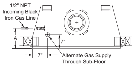
Figure 15 - Manual Shutoff Valve Installation
