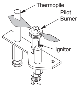
Figure 38 - Correct Pilot Flame Pattern
