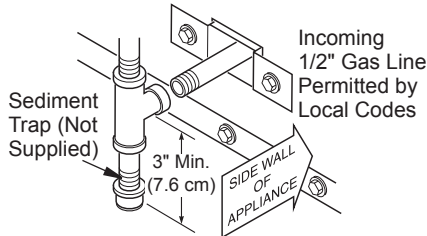
Figure 17 - Sediment Trap
