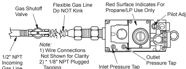
Figure 18 - Connecting Flexible Gas Line to Millivolt Valve
