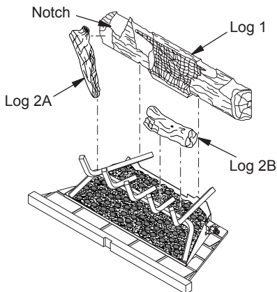
Figure 26 - Installing Logs 1, 2A and 2B
