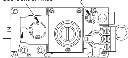
Figure 36 - Control Knob in the PILOT position
