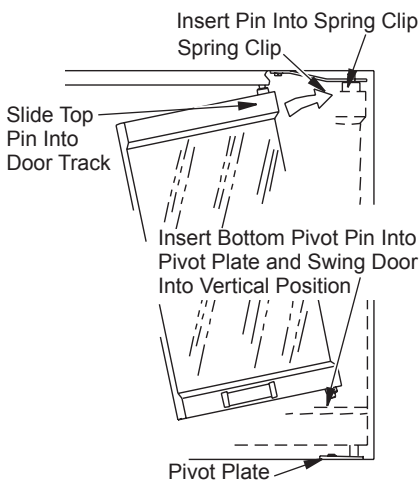
Figure 32 - Installing Optional Glass Door
