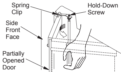
Figure 33 - Adjusting Glass Doors
