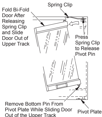
Figure 34 - Removing Glass Doors
