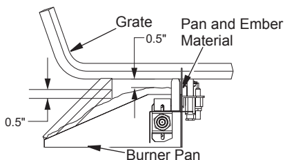
Figure 21 - Pan and Ember Material Clearances
