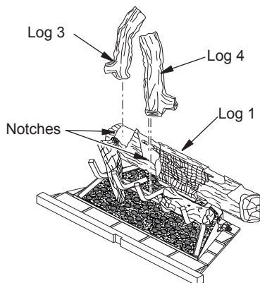
Figure 27 - Installing Logs 3 and 4
