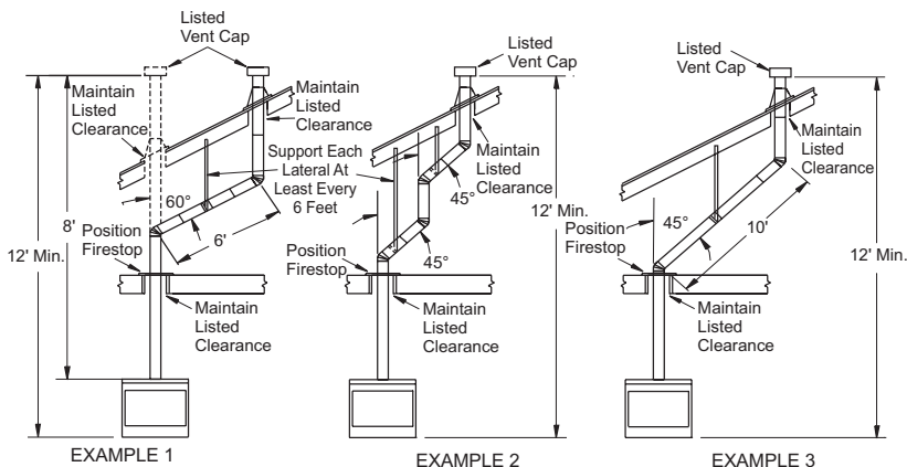
Figure 9 - Typical B-Vent Configuration
