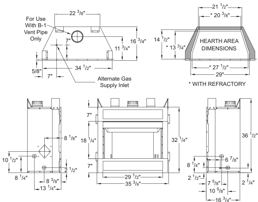
Figure 2 - Appliance Dimensions
