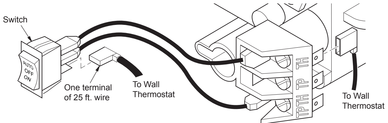
Figure 1 - Connecting Wire Terminals
